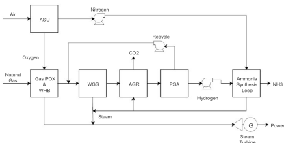
Figure 4. Grannus Process™ simplified process flow diagram.
